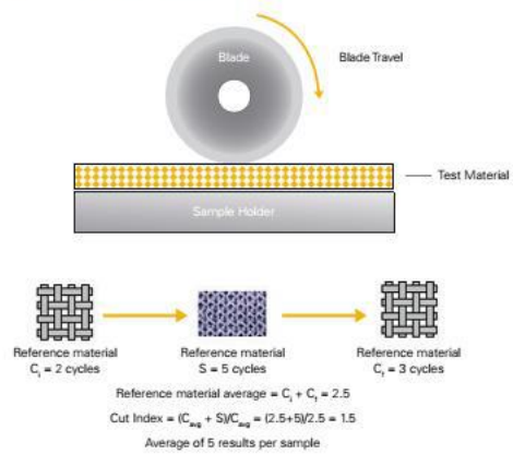
Figure 2. EN 388 test method
