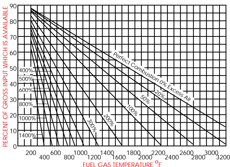
PERCENT AVAILABLE HEAT WITH VARIOUS FLUE GAS TEMPERATURES AND VARIOUS AMOUNT OF EXCESS AIR
