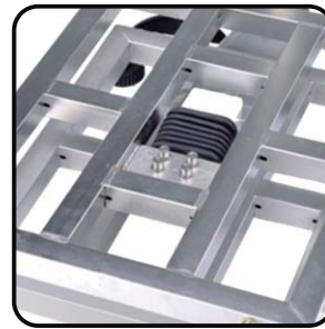
Shock-Guard overload protection
