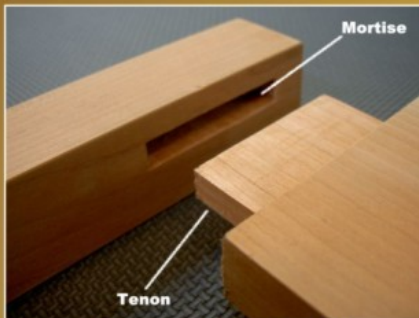
Mortise and Tenon Joinery
